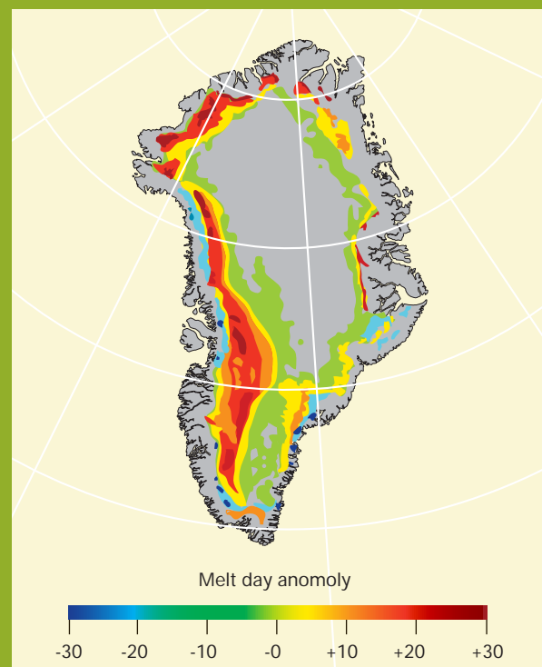
Figure 7. 2011 deviation from mean number of melt days on Greenland over the period 1979-2010
