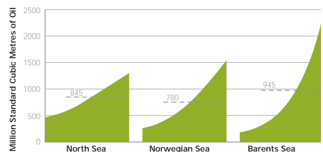
Figure 8. Range of estimates for undiscovered hydrocarbon resources in the North, Norwegian and Barents Seas
