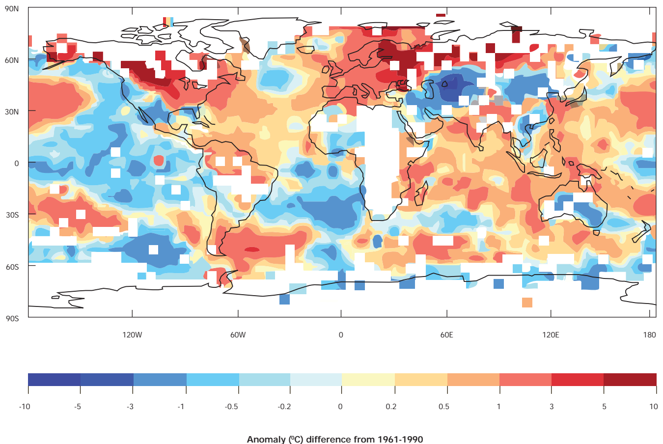
Figure 2. Surface temperature anomalies compared to 1961-1990 baseline
