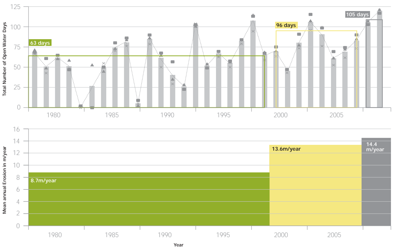
Figure 5. Increase in average number of ice-free days in the Beaufort Sea compared to rates of coastal erosion
