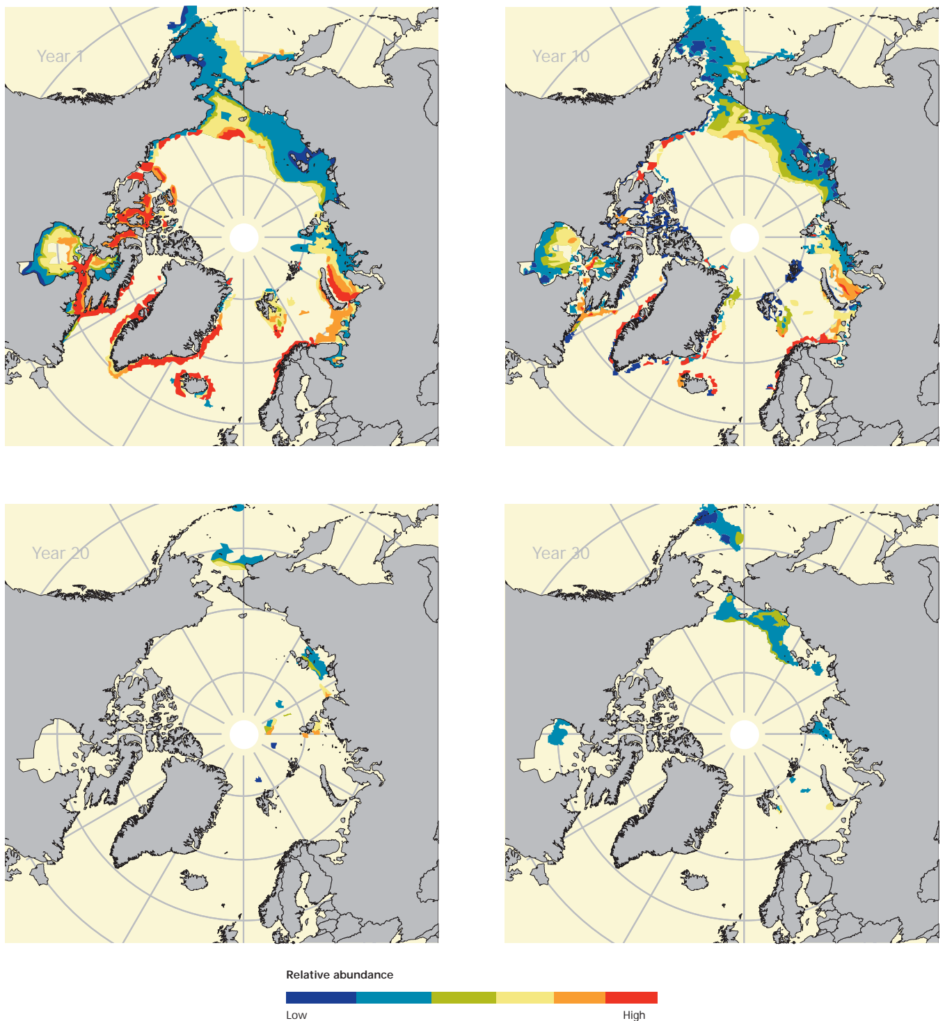
Figure 11. Modelled changes in distributions of Arctic cod over the next 30 years
